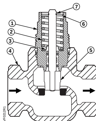
Normally Open
