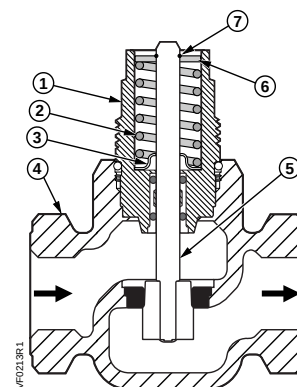
Normally Closed
